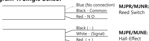
Diagram 1: Single Sensor
