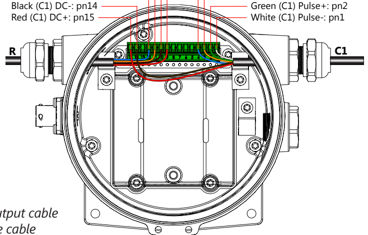
Remote Display
