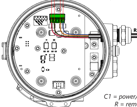
Remote Meter
