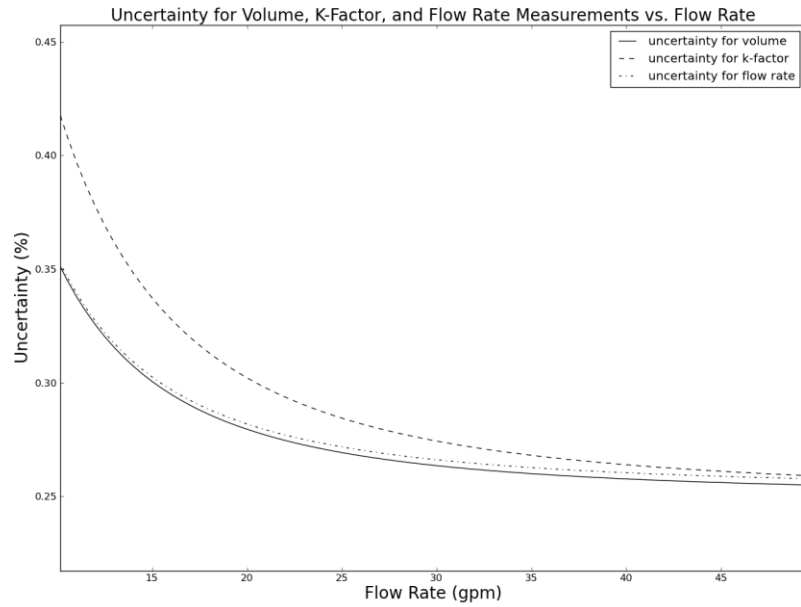
Figure 1 This figure illustrates combined uncertainty volume, k-factor, and flow rate measurements versus flow rate. Coverage factor was two.
