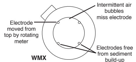
Better Installation: Improved accuracy results from unimpeded electrodes.
