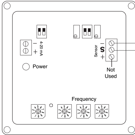
A055W Pulse-to-Analog Converter
