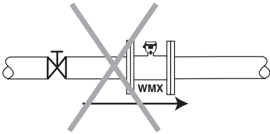
Possible Problem: Post-valve cavitation can create air pocket
