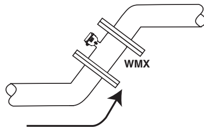
Better Installation: Allows air to bleed off
