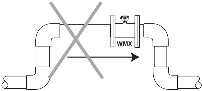
Possible Problem: Allows air pockets to form at sensor
