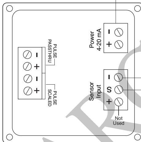
FT420W Remote Rate/Total Display
