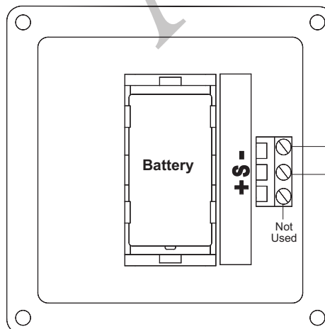
DL75W Data Logger
